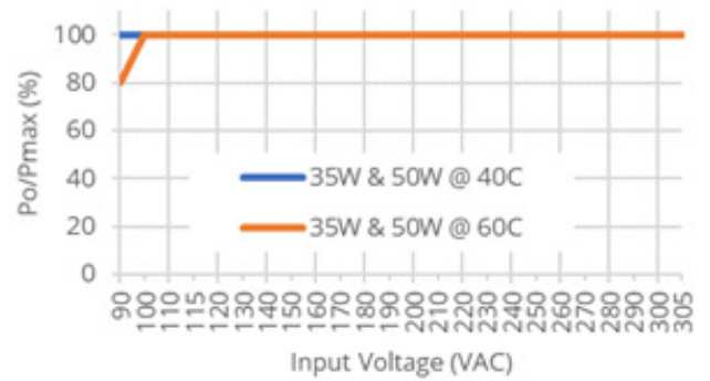
Output Power vs Input Voltage
