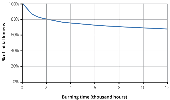
Lumen maintenance CMH G12 150W 4200K
