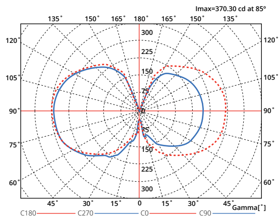
Vertical plane polar intensity curve CMH G12 35W
