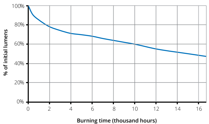
Lumen maintenance CMH G12 35W 3000K
