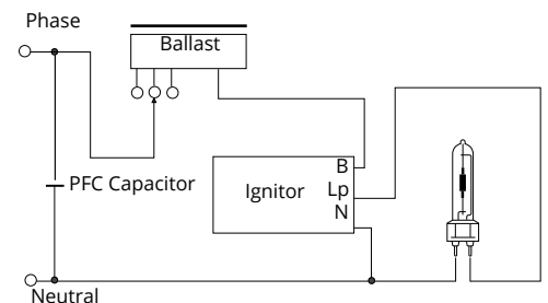
Typical superimposed ignitor circuit
