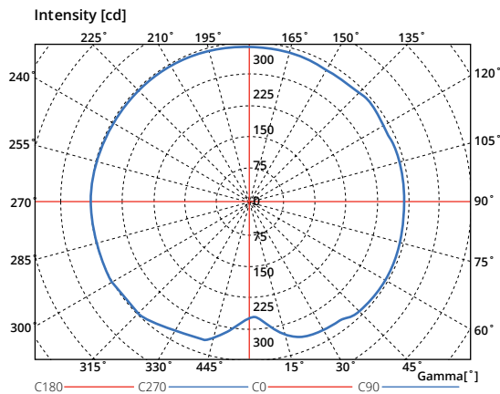
Horizontal plane polar intensity curve CMH G12 35W
