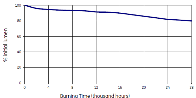
Lumen maintenance of HPS Lucalox™ HO lamps (100 -400W)
