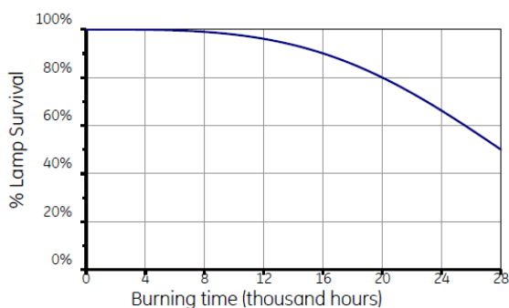
Survival rate of HPS Lucalox™ HO lamps (100 -400W)
