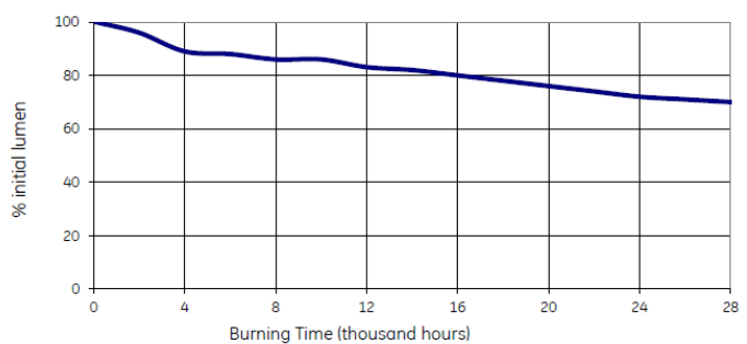
Lumen maintenance of HPS Lucalox™ HO lamps (70W)
