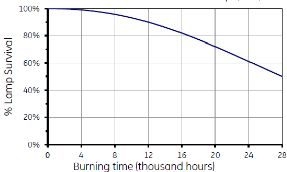
Survival rate of HPS Lucalox™ HO lamps (70W)
